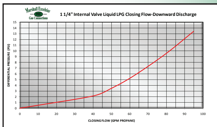
1-1/4" MNPT x 4 Bolt Flange Internal Valve
