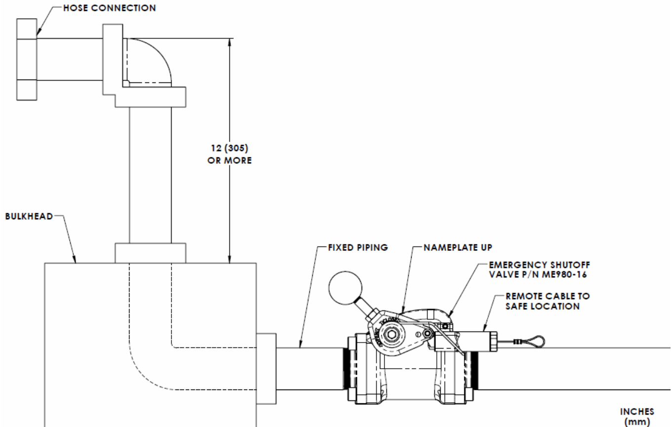
Figure 1: Typical Installation of ME980 Series Using Remote Cable Release
