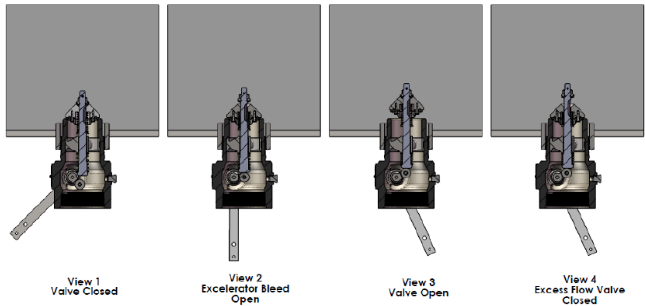
Figure 1: Operational Schematic
