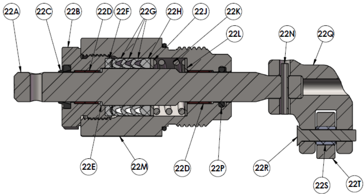
Gland Assembly
