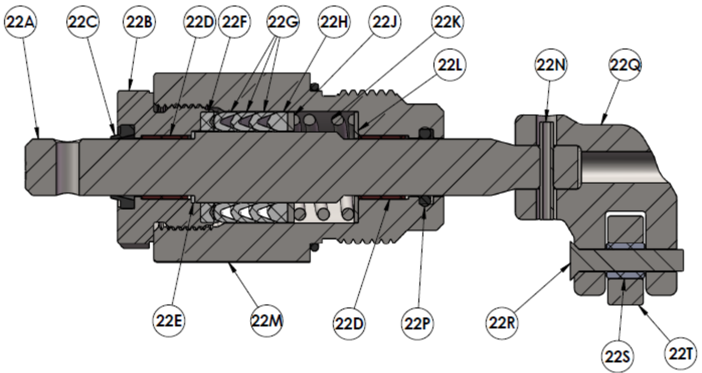
Gland Assembly
