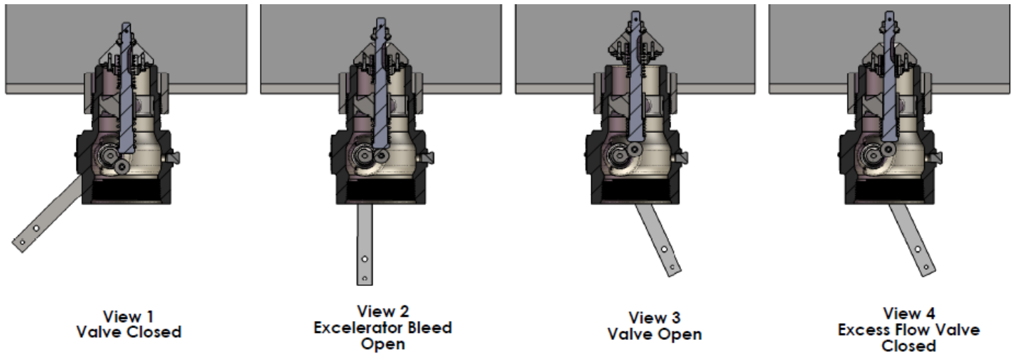
Figure 1: Operational Schematic
