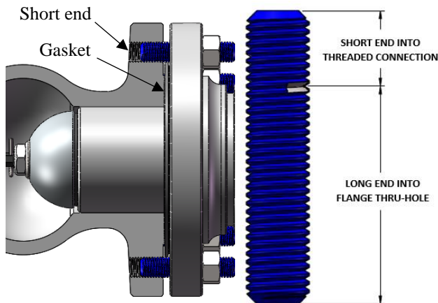
Figure 3: Thread-mount Stud installed
