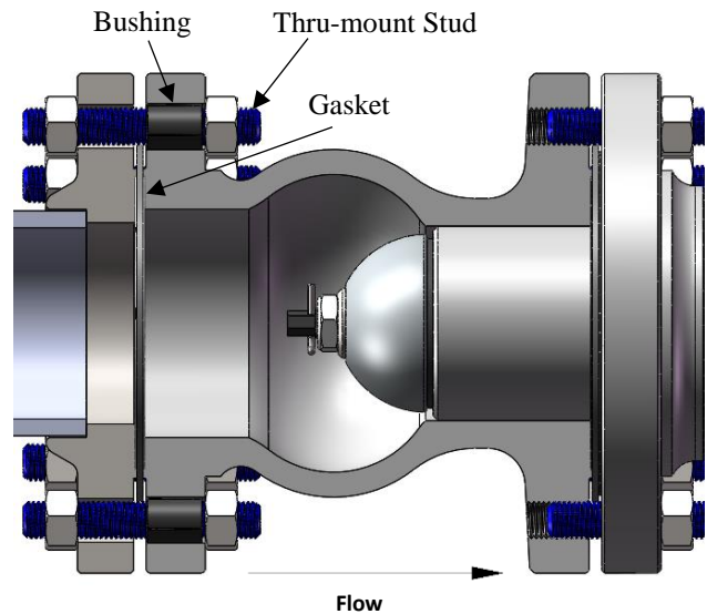
Figure 4: Final Installation
