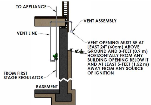
Figure 4: Basement Installation
