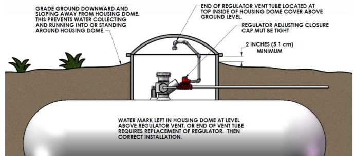
Figure 5: Underground Installation
