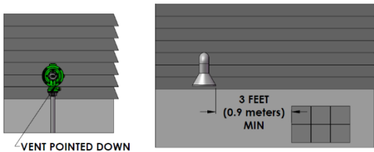
Figure 2: Regulator with Vent Pointed Down
