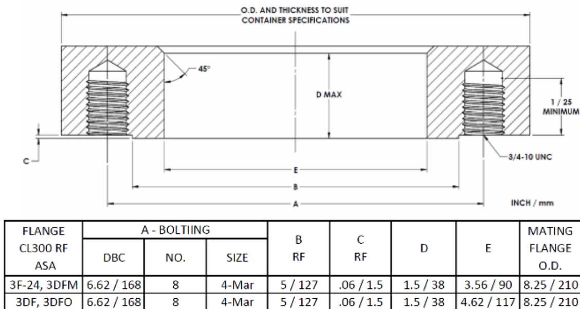
FIGURE 1: TANK FLANGE DIMENSIONS
