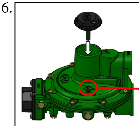
6. Install Dust Cap into Body. Deface UL Logo on Body.
