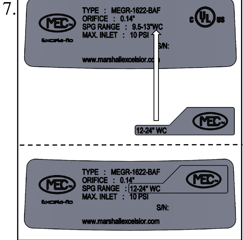
7. Install Spring Range Label onto current Label as shown
