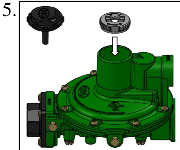
5. Install Spring Retainer into Body. Set to desired outlet pressure
