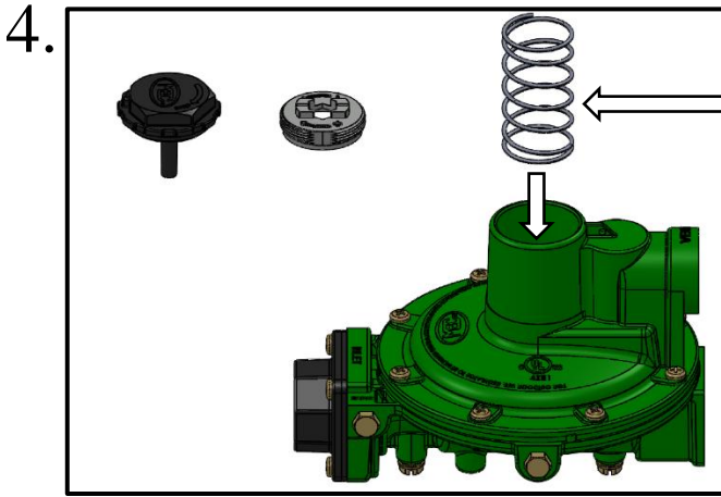
4. Install Spring into Body.
