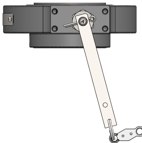
Figure 3: Fuse Assembly
