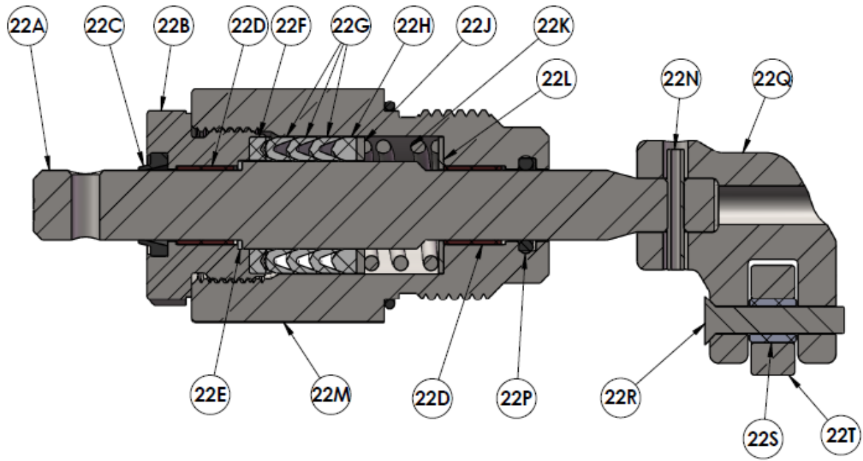
Gland Assembly
