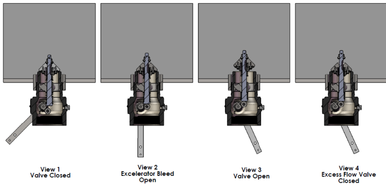
Figure 1: Operational Schematic
