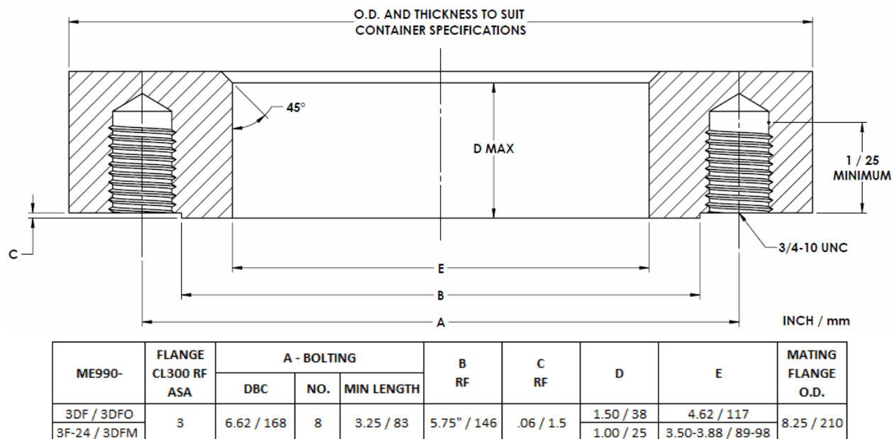
FIGURE 1: TANK FLANGE DIMENSIONS
