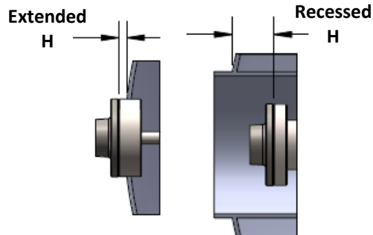
Outer Flange
