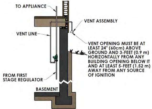
Figure 4: Basement Installation
