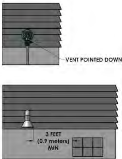
Figure 2: Regulator with Vent Pointed Down
