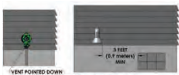
Figure 2: Regulator with Vent Pointed Down
