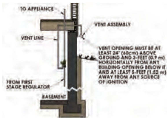
Figure 4: Basement Installation
