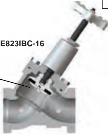
Integrated Back Check Feature
